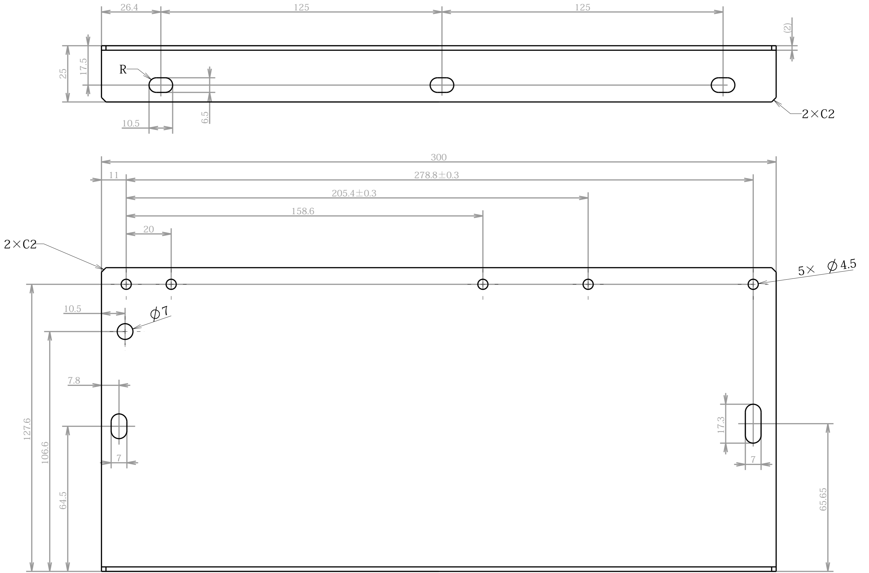
Fixing angle for upright setting B
