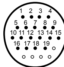
CN20 pin layout
