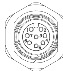
Pin assignment on Ethernet connector
