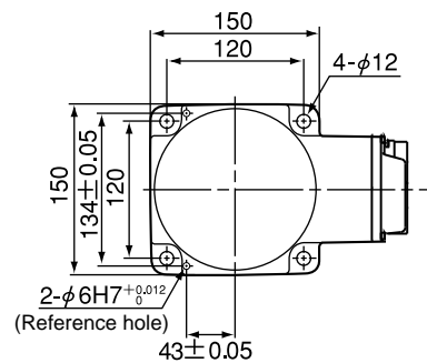
Base mounting dimensions
