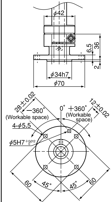
Flange (option) mounting face
