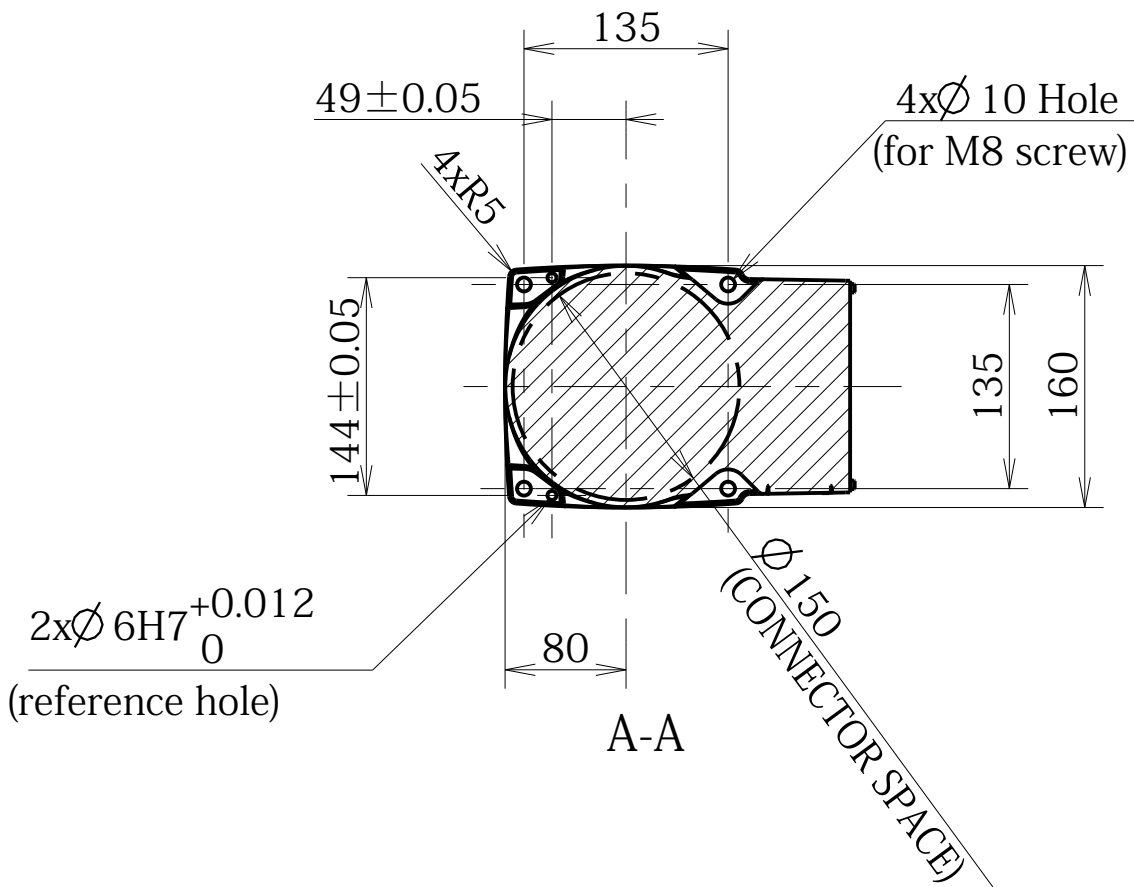
Detailed drawing of base mounting face
