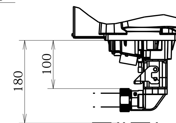
Cable space Angle Connector Type
