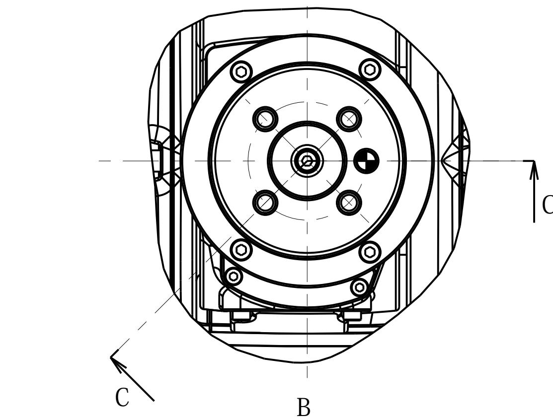
Detailed drawing of end-effector mounting face
