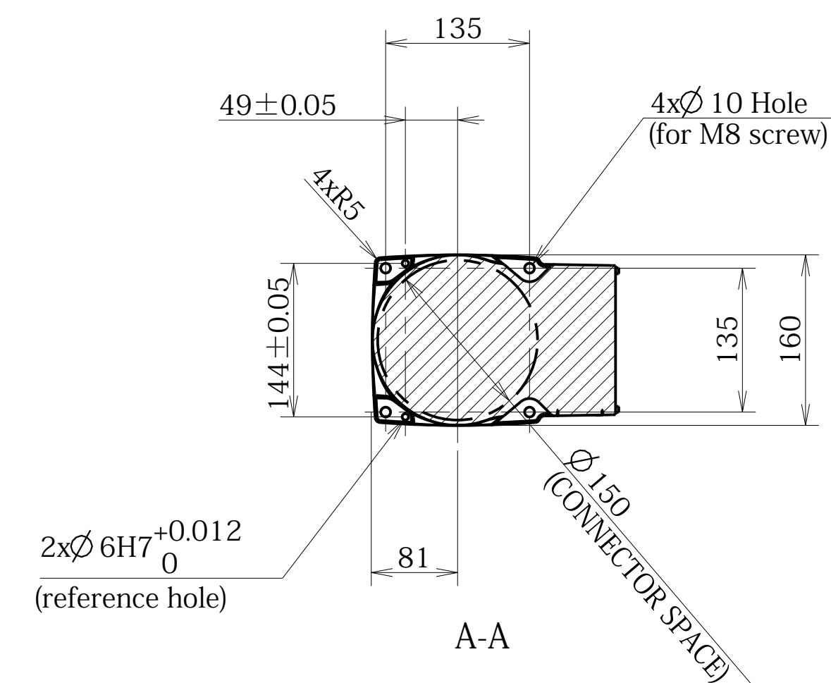
Detailed drawing of base mounting face
