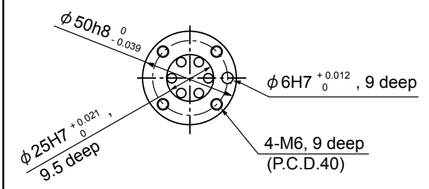
Detailed drawing of end-effector mounting face (View: A)
