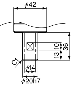
Detailed drawing of hand mounting face (Viewed from D)
