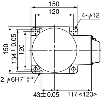
Base mounting dimensions
