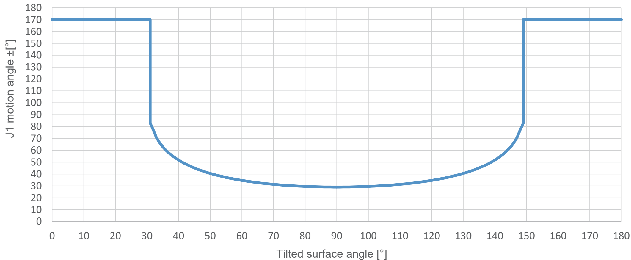
VMB-2518 J1's range of motion angle determined by the angle of a tilted mounting surface
