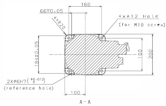
Detailed drawing of base mounting face
