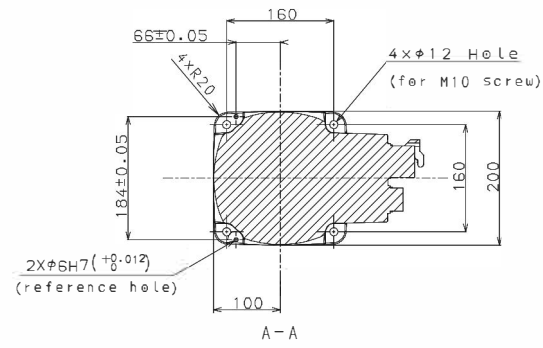
Detailed drawing of base mounting face
