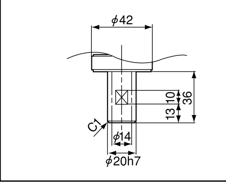
Detailed drawing of hand mounting face (Viewed from D)
