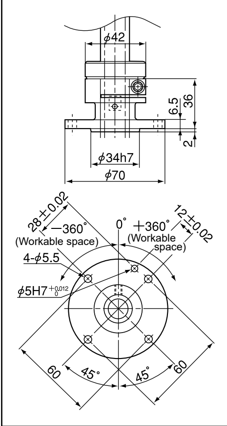
Flange (option) mounting face
