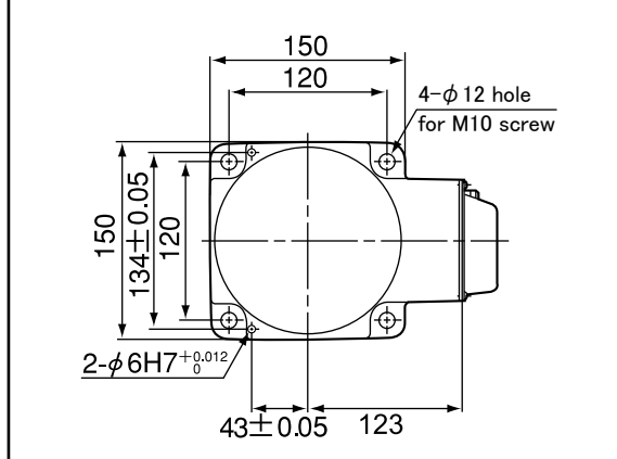
Base mounting dimensions
