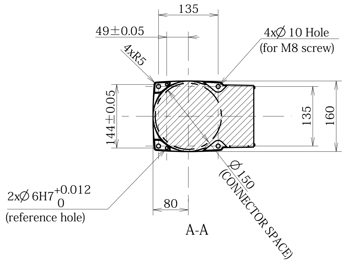
Detailed drawing of base mounting face
