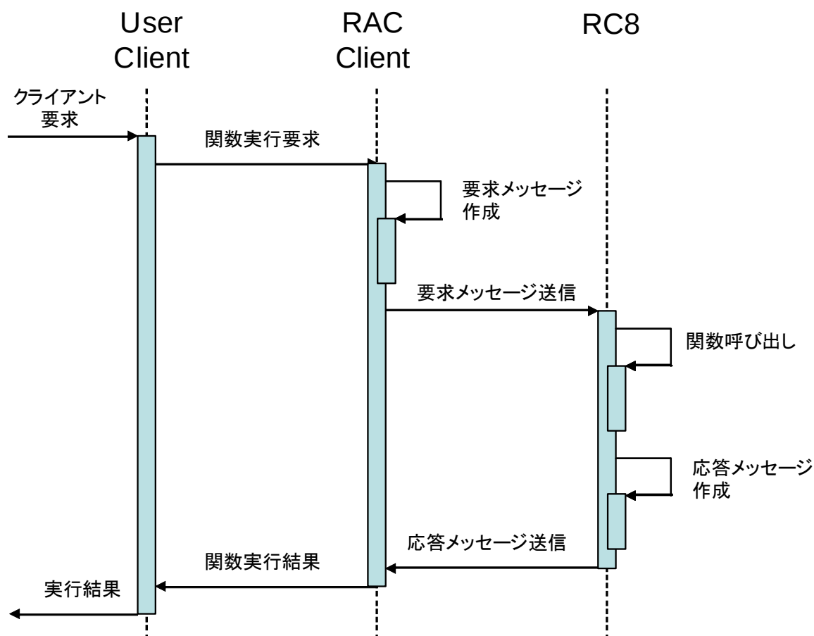
Figure3-1 Communication sequence
